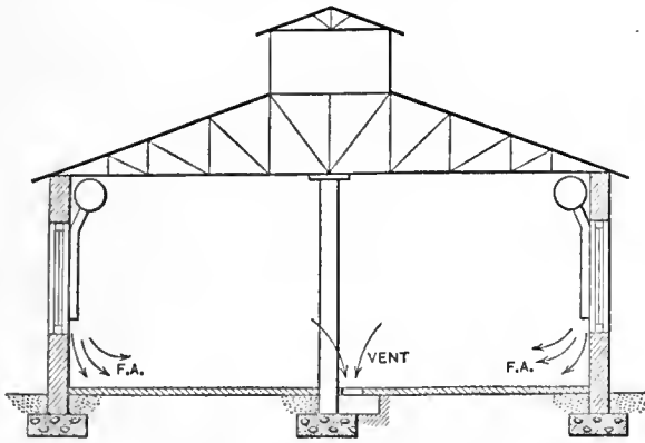
FIG. 2. FOR FOUNDRIES THE ARRANGEMENT OF SUPPLY AND EXHAUST DUCTS HERE SHOWN WILL PRODUCE GOOD RESULTS
